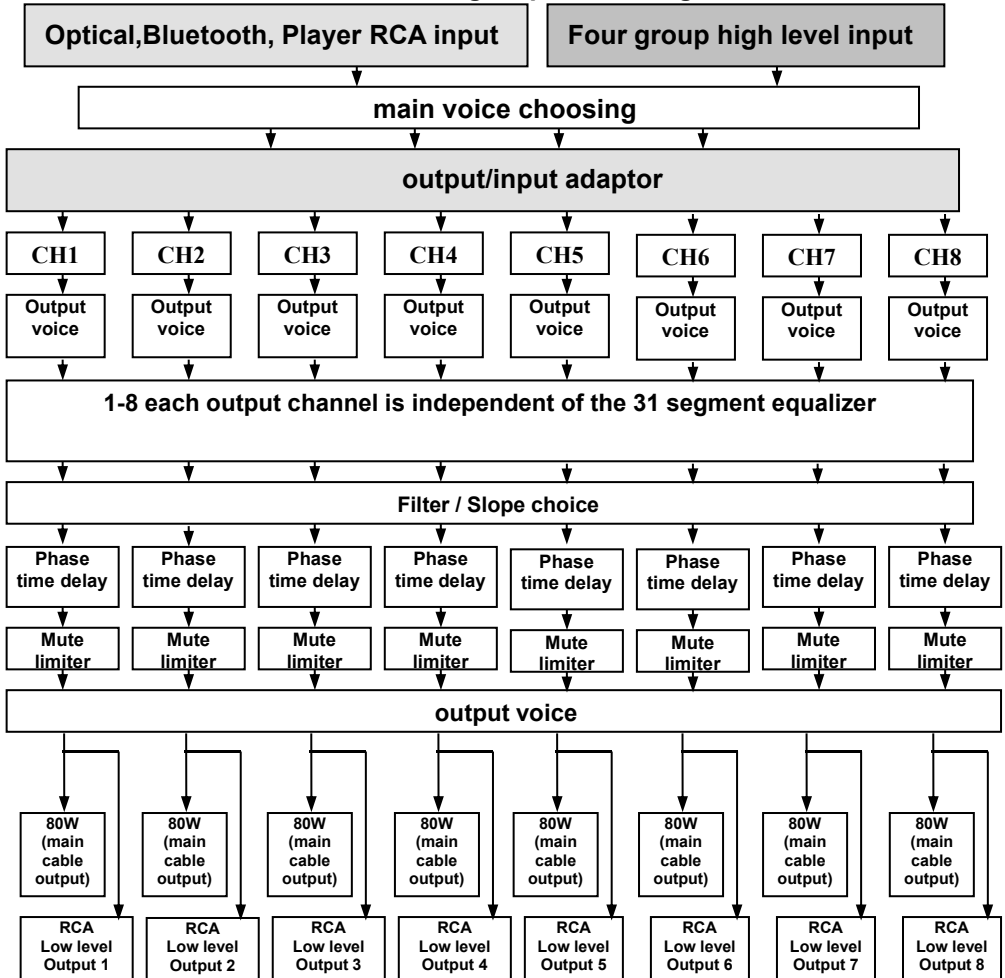
Main audio signal process diagrams
